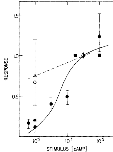
FIGURE 6 Dose-response curves for concentration steps originating at zero. Data from several experiments (different symbols) were combined by normalizing to responses to 0 – 10^{-6} M steps. Responses were total [ ^3 H]cAMP released within 8 min of stimulus application. Error bars indicate range of integrated responses. Closed symbols represent responses monitored at flow rates of 1 drop/4–5 seconds; open symbols represent responses monitored at 1 drop/30 s in the presence of 2 mM DTT.
