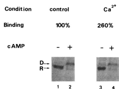
FIG. 2. Effect of \text{Ca}^{2+} on receptor occupancy and receptor modification. Cells were incubated in the absence (control) or presence of 10 mM \text{CaCl}_2 for 10 min. Receptor modification was induced by a 15-min incubation with 0.5 \mu\text{M} cAMP + DTT; proteins were separated by SDS-PAGE and Western blot analysis with an antiserum directed against the purified receptor. Lanes 1 and 2 are samples from control cells; lanes 3 and 4 from cells incubated with 10 mM \text{Ca}^{2+} . Lanes 1 and 3 are from unstimulated cells (R, unmodified form of the receptor); lanes 2 and 4 are from cells stimulated with cAMP + DTT (D, modified form). [ ^3\text{H} ]cAMP binding was determined as described under "Experimental Procedures." 100 \pm 13 represents binding in control cells, and 260 \pm 11 binding in the presence of \text{Ca}^{2+} .
