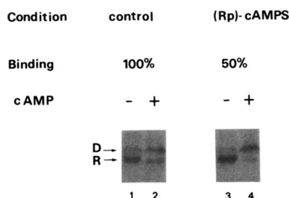
FIG. 3. Effect of ( R_p )-cAMPS on down-regulation and receptor modification. cAMP receptors were down-regulated by incubating cells for 15 min with 100 \mu\text{M} ( R_p )-cAMPS. Control cells were not exposed to ( R_p )-cAMPS. Cells were washed with ice-cold Mes, and incubated for 15 min with 0.5 \mu\text{M} cAMP + DTT. Lanes 1 and 2, control cells; lanes 3 and 4, cells with down-regulated receptors; lanes 1 and 3, cells immediately after washing in Mes buffer; lanes 2 and 4, cells after a subsequent incubation with 0.5 \mu\text{M} cAMP + DTT. cAMP binding was measured immediately after washing of cells with Mes buffer. Cells with down-regulated receptors by ( R_p )-cAMPS show 50% \pm 8 of [ ^3\text{H} ]cAMP binding.
