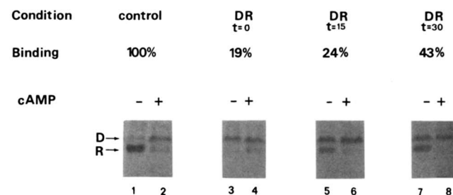
FIG. 4. Effect of cAMP on down-regulation and shifting. D. discoideum cells were incubated for 15 min in the absence or presence of 1 \mu\text{M} cAMP and 10 mM DTT, washed (at 0 ^\circ\text{C} ), resuspended (at 20 ^\circ\text{C} ) in Mes buffer. Cells were divided into three portions, which were used after 0, 15, and 30 min for the determination of cAMP binding or a subsequent incubation with 0.5 \mu\text{M} cAMP + DTT. Lanes 1 and 2, control cells; lanes 3 and 4, cells with down-regulated receptors at t=0 ; lanes 5 and 6, 7, and 8, cells with down-regulated receptors, respectively, at 15 and 30 min after removal of the stimulus. Lanes 1, 3, 5, and 7 before and lanes 2, 4, 6, and 8 after the subsequent incubation with 0.5 \mu\text{M} cAMP + DTT. Binding data represent cAMP binding to the down-regulated receptors at t_0 = 19 \pm 4\% , t_{15} = 24 \pm 5\% , and t_{30} = 43 \pm 8\% .
